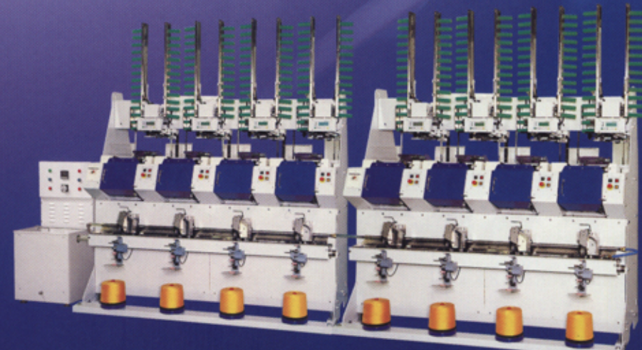
TN-35A全自動高速繞線機-Y型管 Automatic High Speed Cross Cone Winder(King Spool Type)
