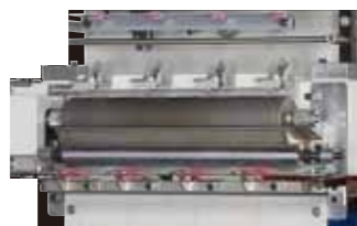
上油裝置 Lube system
