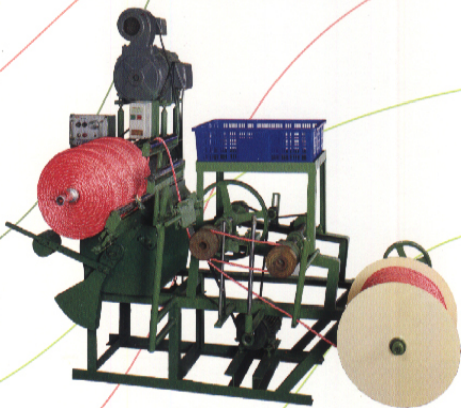
TN-01H 臥式繞線機 Horizontal Type Cross Cone Winder
